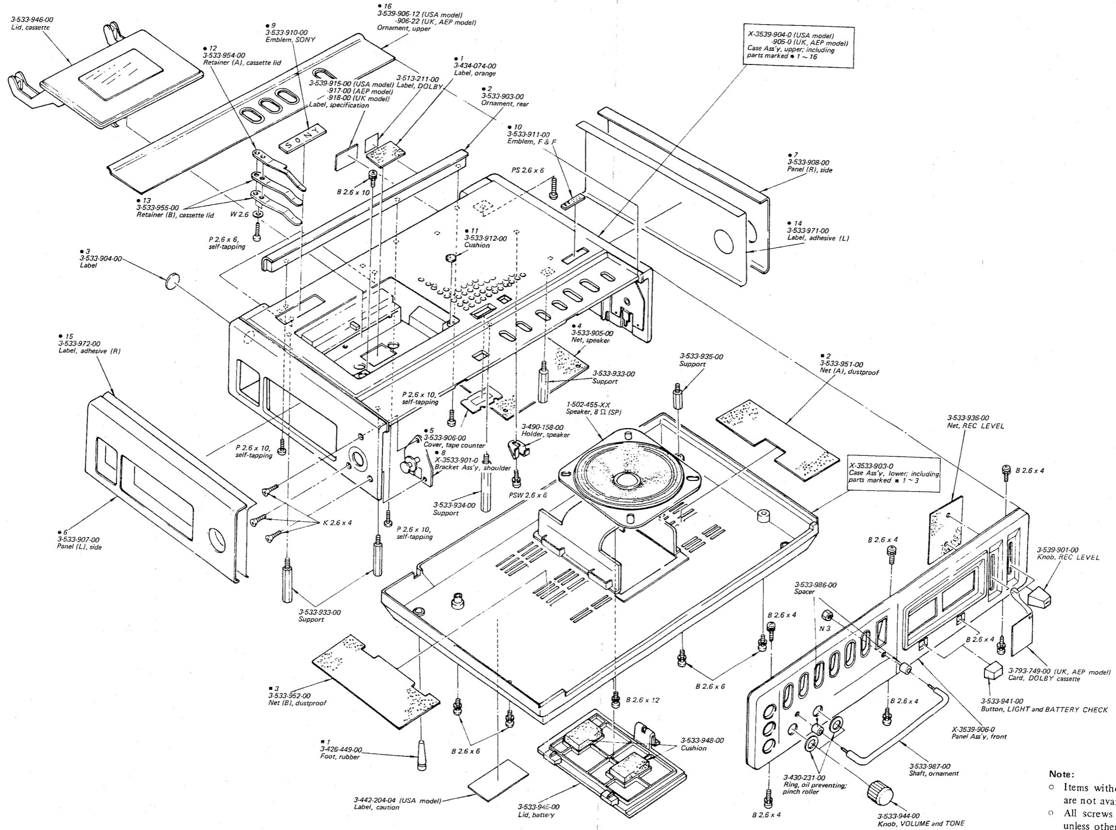
5-1. EXPLODED VIEW (1)
